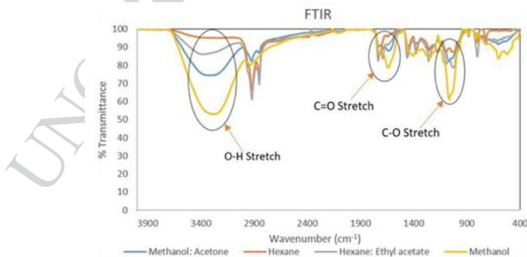
Figure 5: FTIR spectra of Ixora javanica 's flower crude solvent extracts
