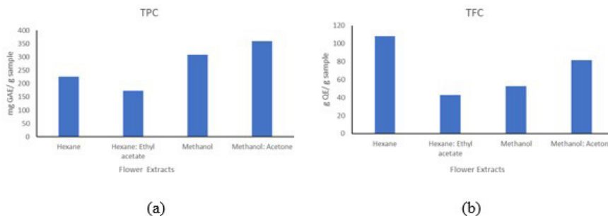
Figure 2: Bioassay of (a) TPC and (b) TFC from different types of solvent Ixora javanica extracts
