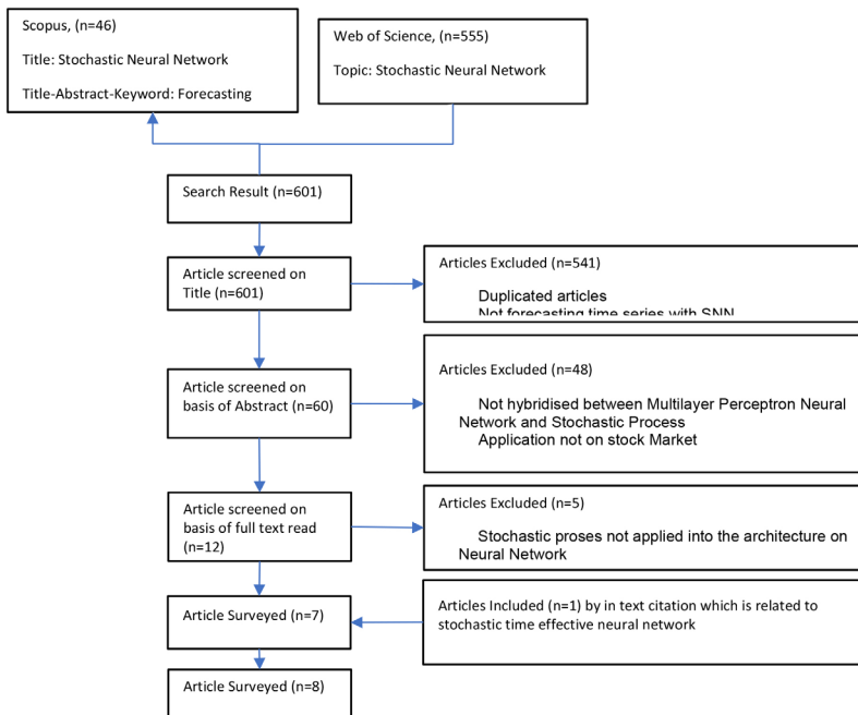
Figure 3: Flow diagram of the selected articles from the database [39] Note: Abbreviation: n, number of systematic reviews
