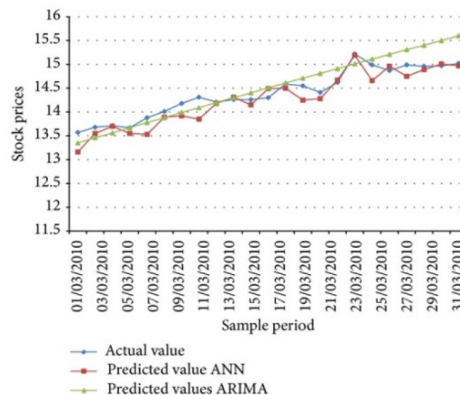
Figure SEQ Figure \* ARABIC \s 1 1: Graph of predicted value of ARIMA and ANN model against actual stock price [17]
